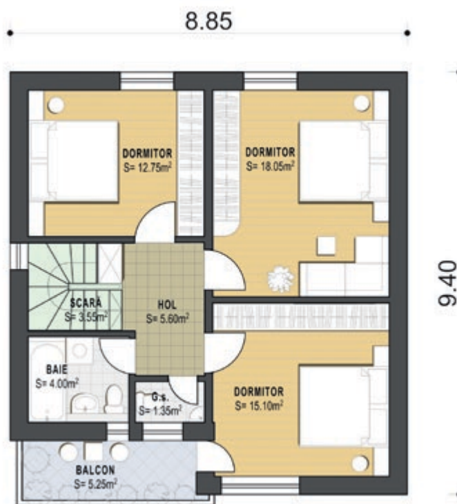
Plan MANSARDĂ
